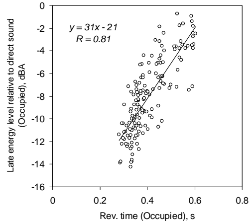
Figure 4: Relation between reverberation times and late energy levels (relative to the direct sound) in occupied classrooms.
